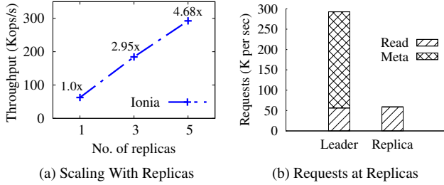
Figure 11: Read Scaling. (a): read-only throughput with varying replicas. (b): meta queries vs. read requests at IONIA's leader with five replicas.
